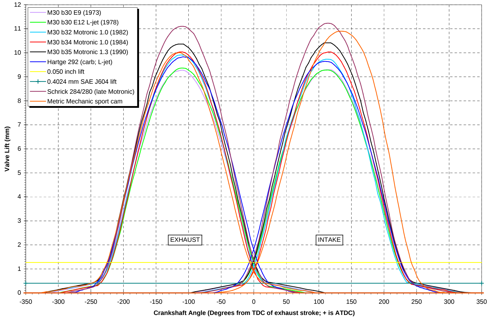
Valve Lift Profile
